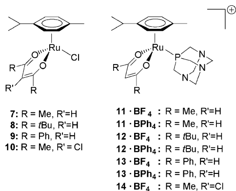
Figure 2. Structures of the neutral complexes 7–10 and the new monocationic PTA derivatives 11–14.
