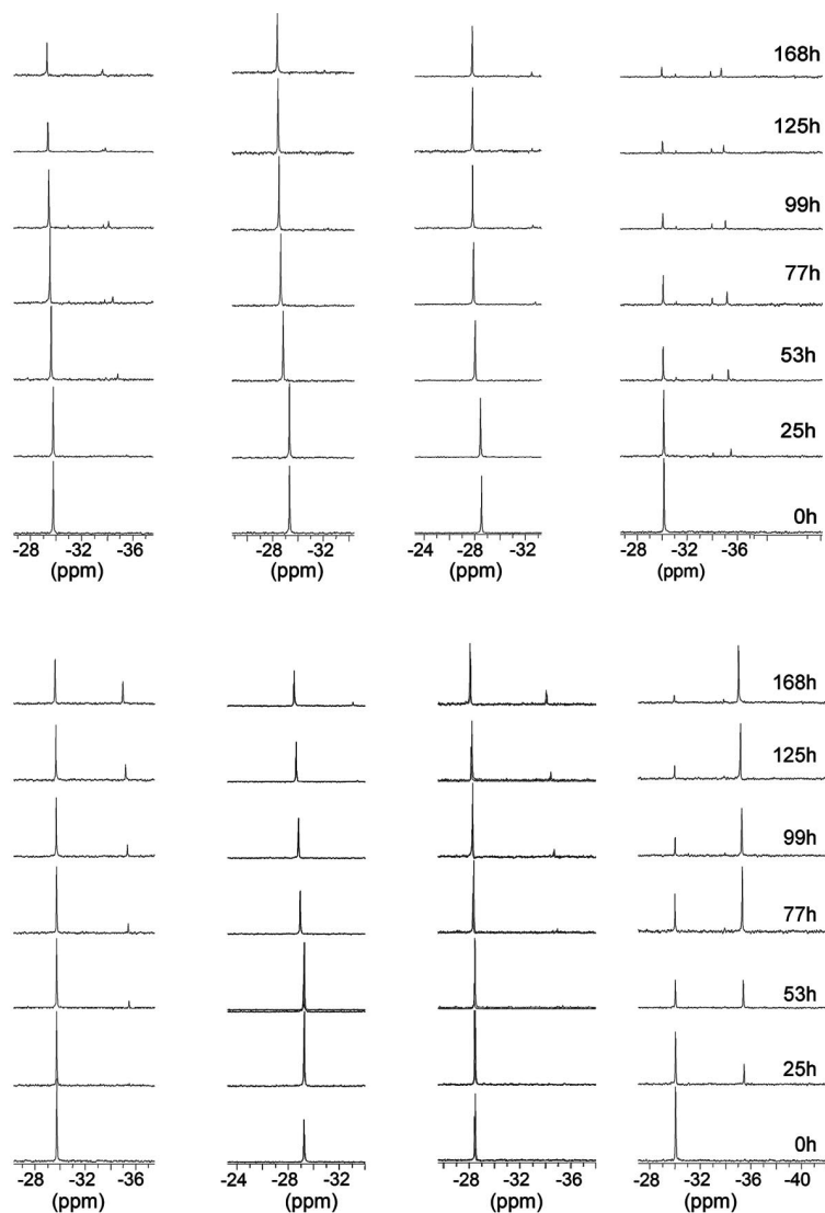
Figure 5. Kinetic hydrolysis experiment at 37 °C: 2.0 mM solution of complex 11 ·BF 4 – 14 ·BF 4 in (top) 5.0 mM NaCl/D 2 O (1% [D 6 ]DMSO) and (bottom) 100 mM NaCl/D 2 O (1% [D 6 ]DMSO).
