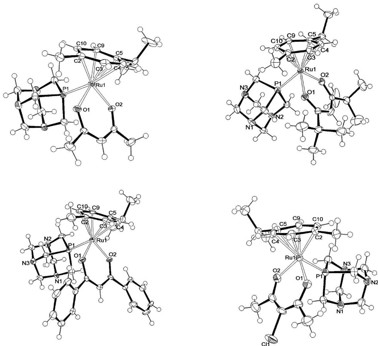
Figure 3. ORTEP plots of 11 · \text{BPh}_4 (top, left), 12 · \text{BPh}_4 (top, right), 13 · \text{BF}_4 (bottom, left) and 14 · \text{BF}_4 (bottom, right) drawn with 50% probability ellipsoids ( \text{BF}_4 and \text{BPh}_4 anions omitted for clarity).
