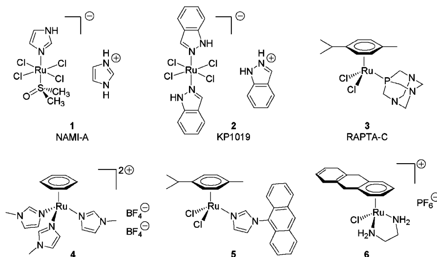
Figure 1. Structures of NAMI-A (1), KP1019 (2), RAPTA-C (3), [\text{Ru}(\eta^6\text{-benzene})(\text{mimid})_3][\text{BF}_4]_2 (4), [\text{Ru}(\eta^6\text{-}p\text{-cymene})(\text{anthraimide})\text{Cl}_2] (5) and [\text{Ru}(\eta^6\text{-tetrahydroanthracene})(\text{ethylenediamine})\text{Cl}][\text{PF}_6] (6).
