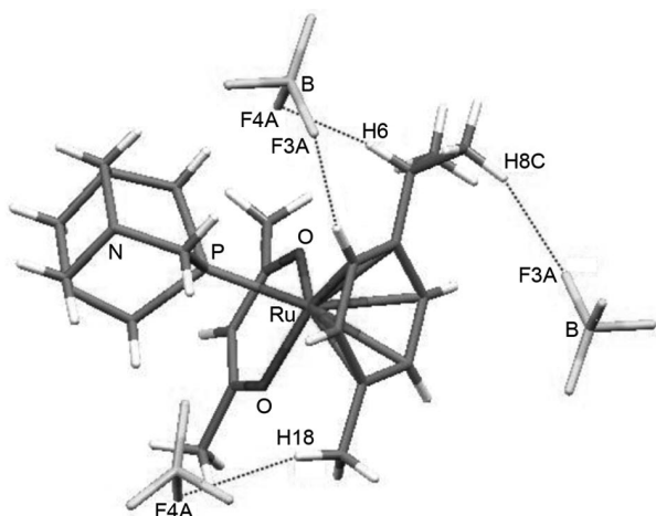
Figure 4. Interactions between the cymene moiety and BF 4 counterions in complex 11 ·BF 4 .
